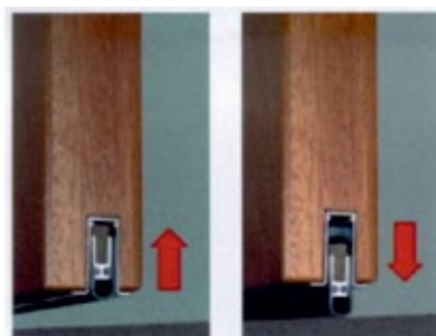
Down sliding door seal for single-leaf door
